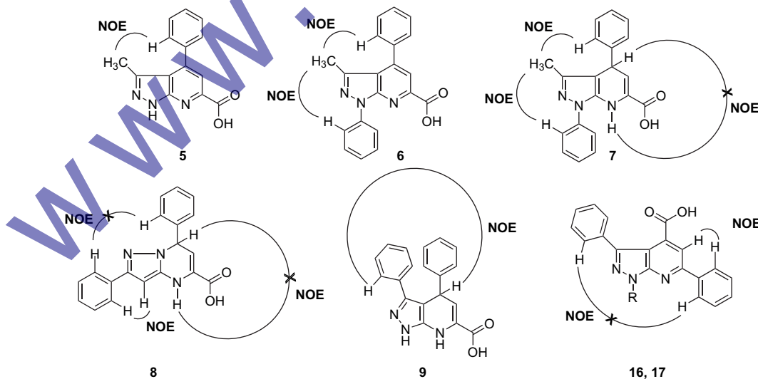
Figure 2. NOE experiments for structure determinations.
